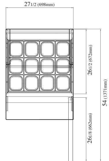
PLAN VIEW
