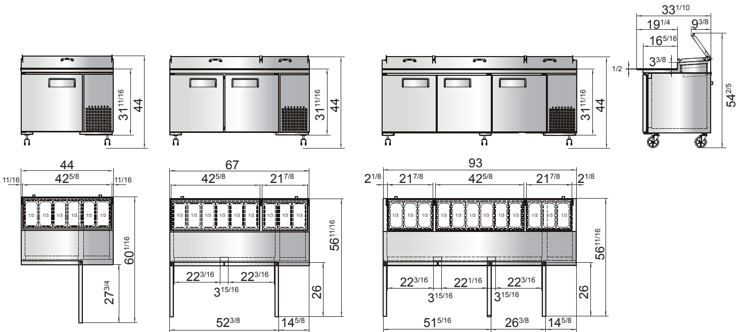
FGA-PZPT-1D-44
