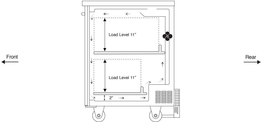
Side View
