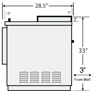
SIDE VIEW (1,2,3 DOORS)
